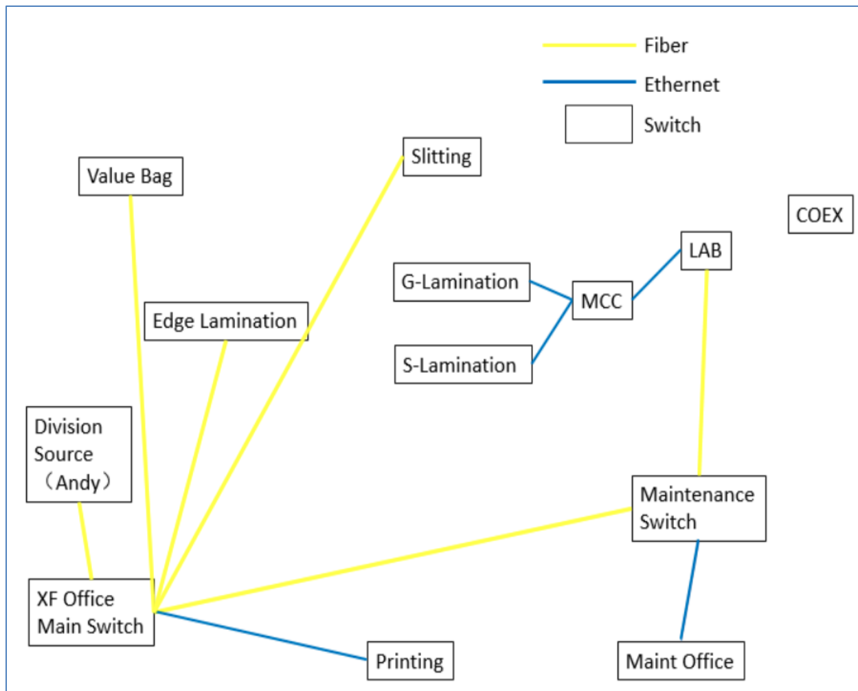
Figure 6-6: XF Network Topology Diagram - XF facility network topology diagram containing yellow fiber-optic links and blue Ethernet connections.
